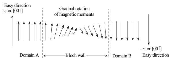
Fig. 8.25: In a Bloch wall the neighboring spin magnetic moments rotate gradually and it takes several hundred atomic spacings to rotate the magnetic moment by 180^\circ .
