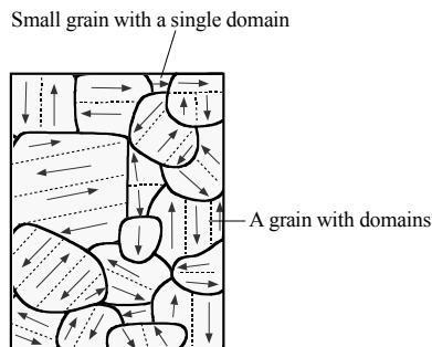
Fig. 8.29: Schematic illustration of magnetic domains in the grains of an unmagnetized polycrystalline iron sample. Very small grains have single domains.
