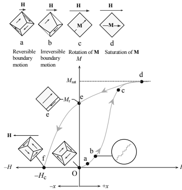
Fig. 8.30: M vs. H behavior of a previously unmagnetized polycrystalline iron specimen. An example grain in the unmagnetized specimen is that at O. (a) Under very small fields the domain boundary motion is reversible, (b) The boundary motions are irreversible and occur in sudden jerks. (c) Nearly all the grains are single domains with saturation magnetizations in the easy directions. (d) Magnetizations in individual grains have to be rotated to align with the field, H . (e) When the field is removed the specimen returns along d to e. (f) To demagnetize the specimen we have to apply a magnetizing field of H_c in the reverse direction.
