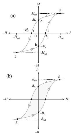
Fig. 8.31: (a) A typical M vs. H hysteresis curve (b) The corresponding B vs. H hysteresis curve. The shaded area inside the hysteresis loop is the energy loss per unit volume per cycle.
