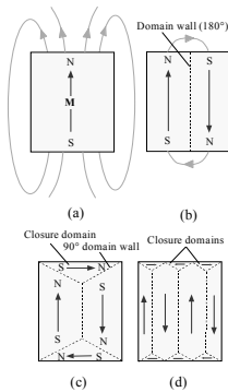
Fig. 8.22: (a) Magnetized bar of ferromagnet in which there is only one domain and hence an external magnetic field. (b) Formation of two domains with opposite magnetizations reduces the external field. There are, however, field lines at
